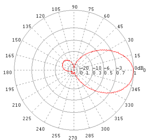
E-Ebene / E-Plane 250 MHz
