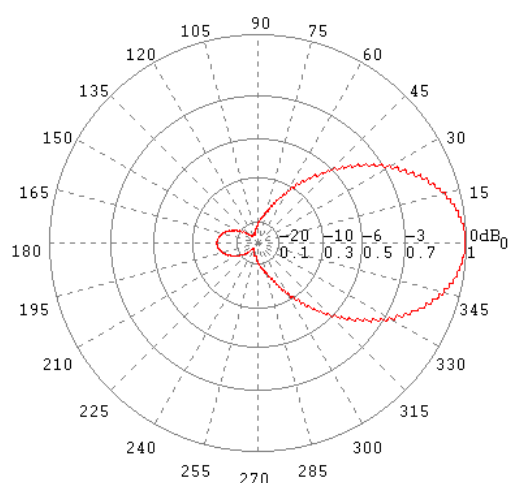
H-Ebene / H-Plane 200 MHz
