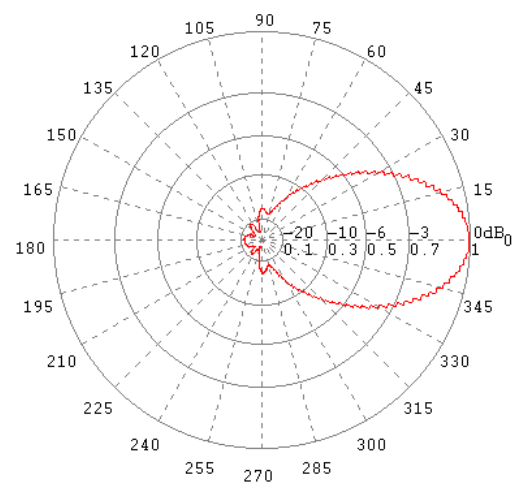
H-Ebene / H-Plane 600 MHz
