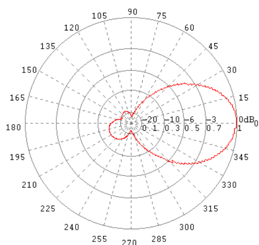
E-Ebene / E-Plane 200 MHz
