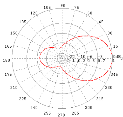
H-Ebene / H-Plane 150 MHz
