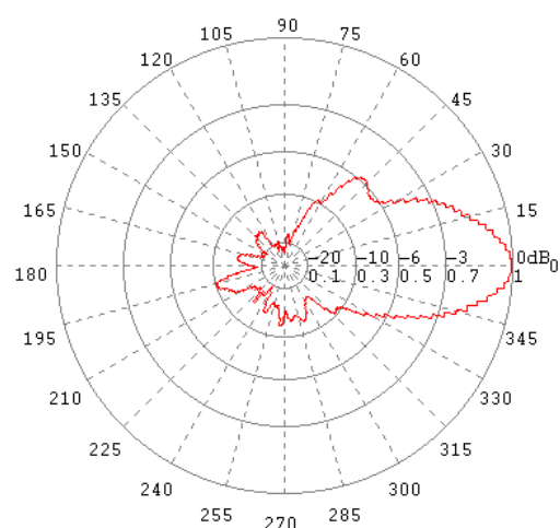
E-Ebene / E-Plane 2500 MHz
