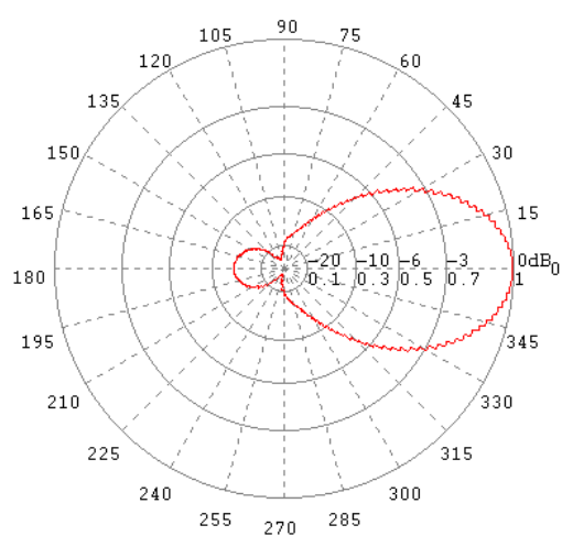
H-Ebene / H-Plane 250 MHz
