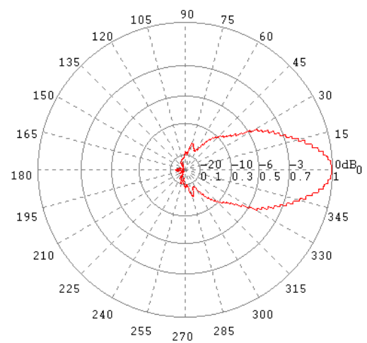
H-Ebene / H-Plane 1500 MHz
