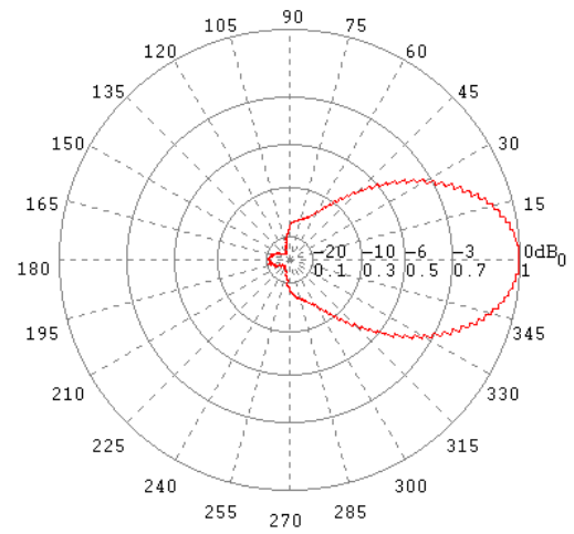
H-Ebene / H-Plane 300 MHz
