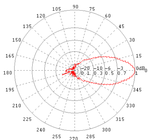
H-Ebene / H-Plane 2500 MHz
