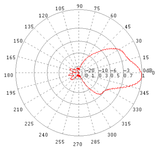
E-Ebene / E-Plane 1500 MHz
